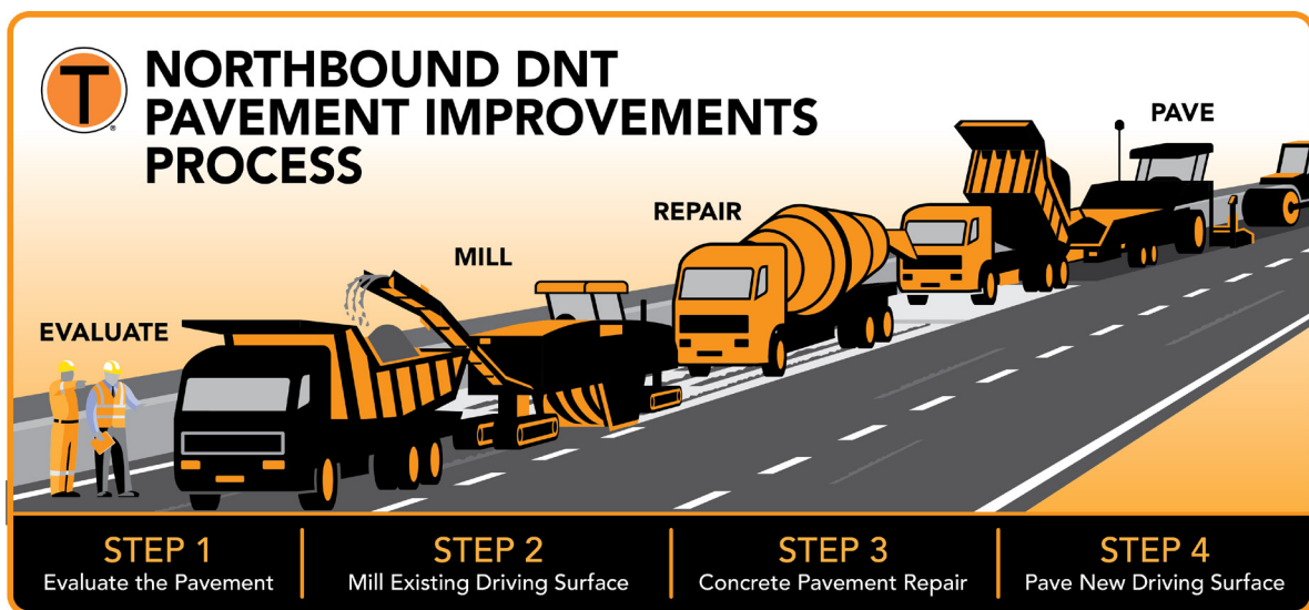
New driving surface and pavement markings on the northbound mainlanes
