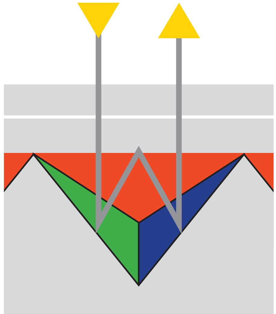
Cube Corner Retroreflection
