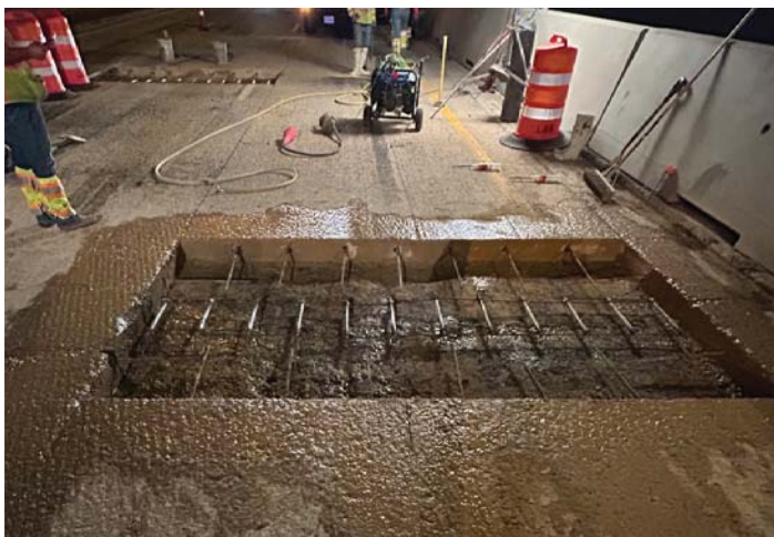
DNT concrete repairs
