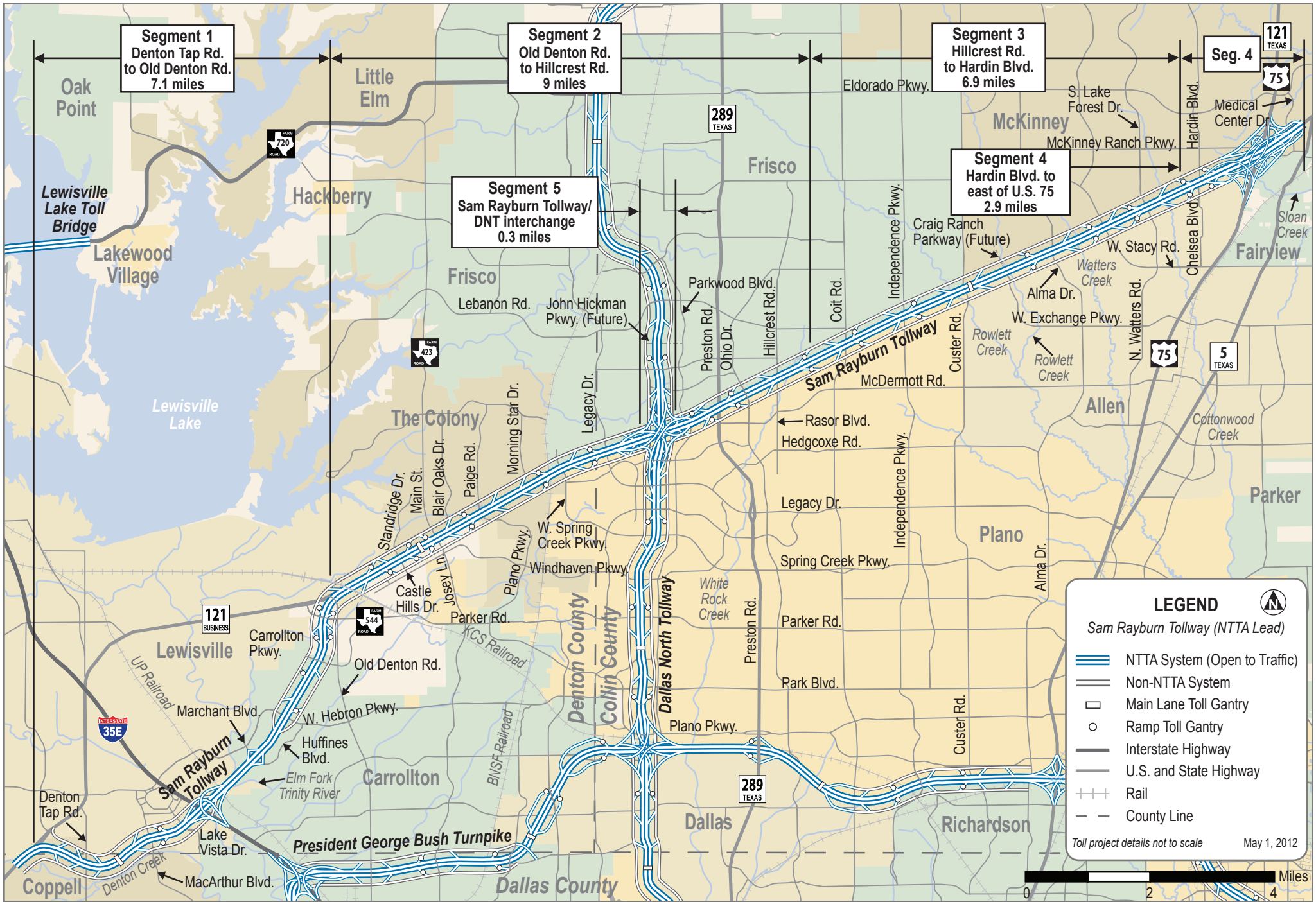
Sam Rayburn Tollway Project Location Map
